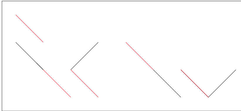
Figure 1: incomplete binary trees with one red edge on the sequence of consecutive left edges leaving the root
